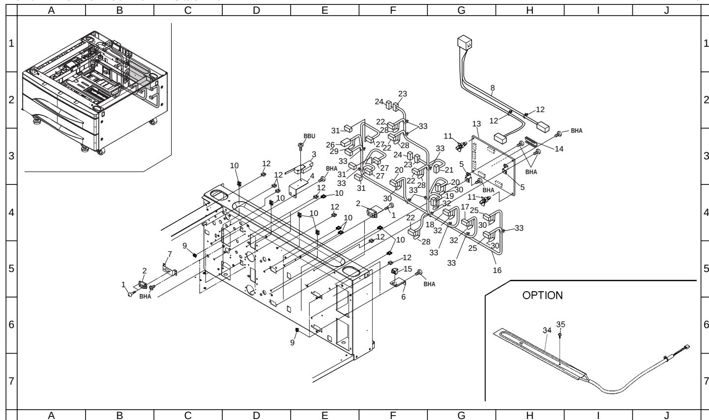
FIG. 6 ELECTRICAL COMPONENTS & OPTION
